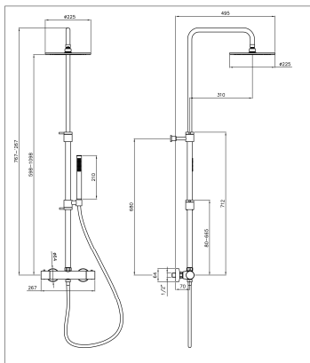
Circular Wall Mounted thermostatic valve with rigid riser, fixed head and shower kit AB4190 v1 © abode home products ltd not liable for continuing improvement and obsolete products, and accordingly we reserve the right to amend specifications without prior notice.
