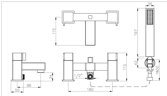
Rapport deck mounted bath shower mixer (hand shower)
