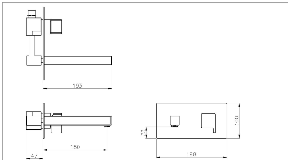
Rapport single lever wall mounted basin mixer
