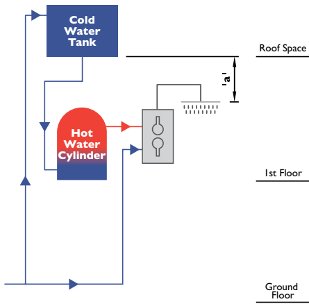
GRAVITY FED CYLINDER - VENTED SYSTEM
